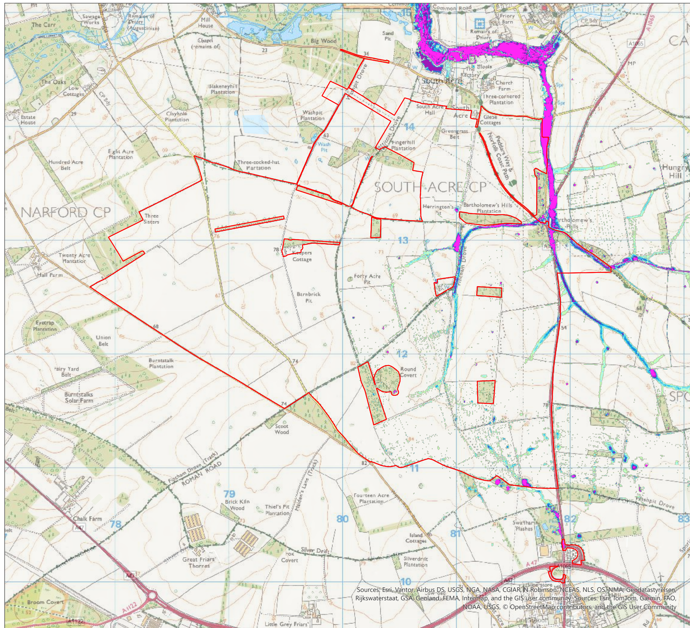
1 % AEP + 40 % CC Flood Depths - Raincloud 2D Modelling Figure A12-1-8
